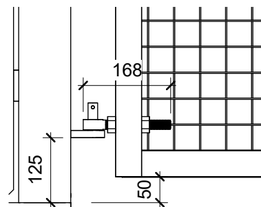
SCALE 1:10
